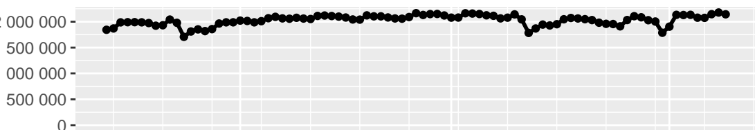
Update pings
