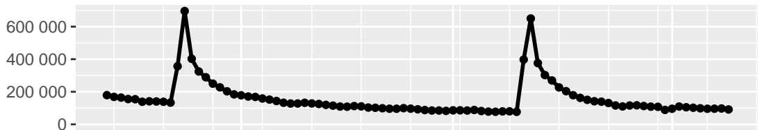
Update requests
